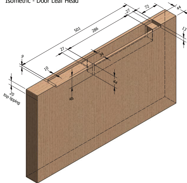
Isometric - Door Leaf Head
