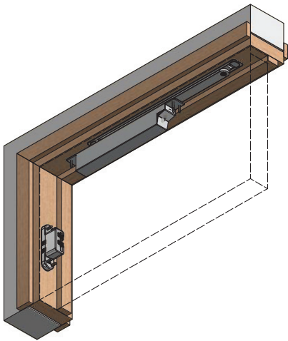
Isometric - Door Head
