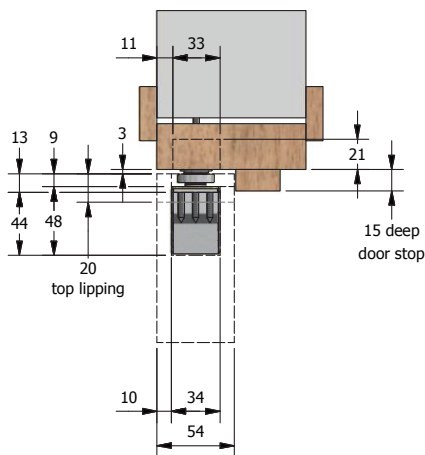
Vertical Section
