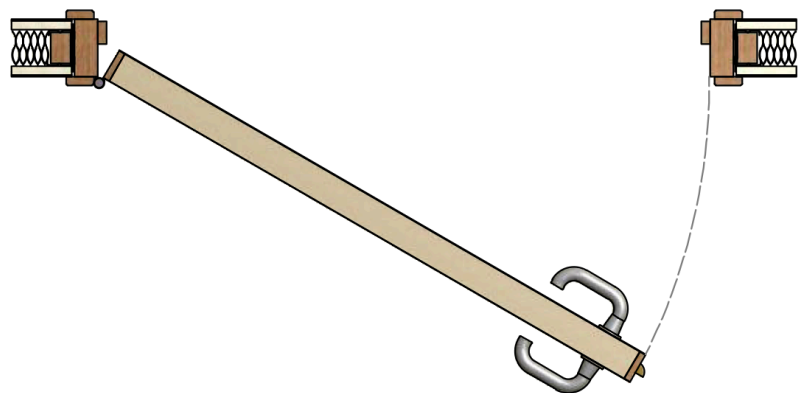
Single Doorset Left-hand opening
