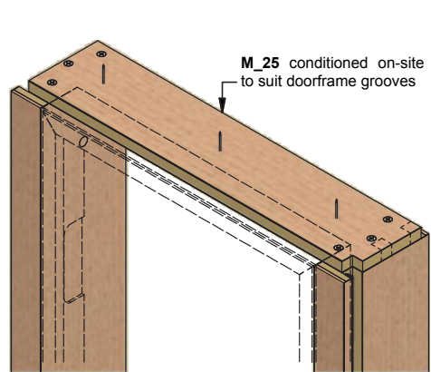
Doorframe Top Right Isometric
