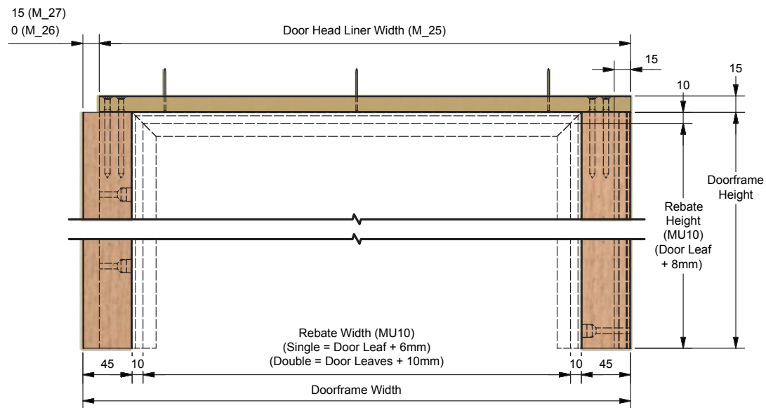
Doorframe Front View
