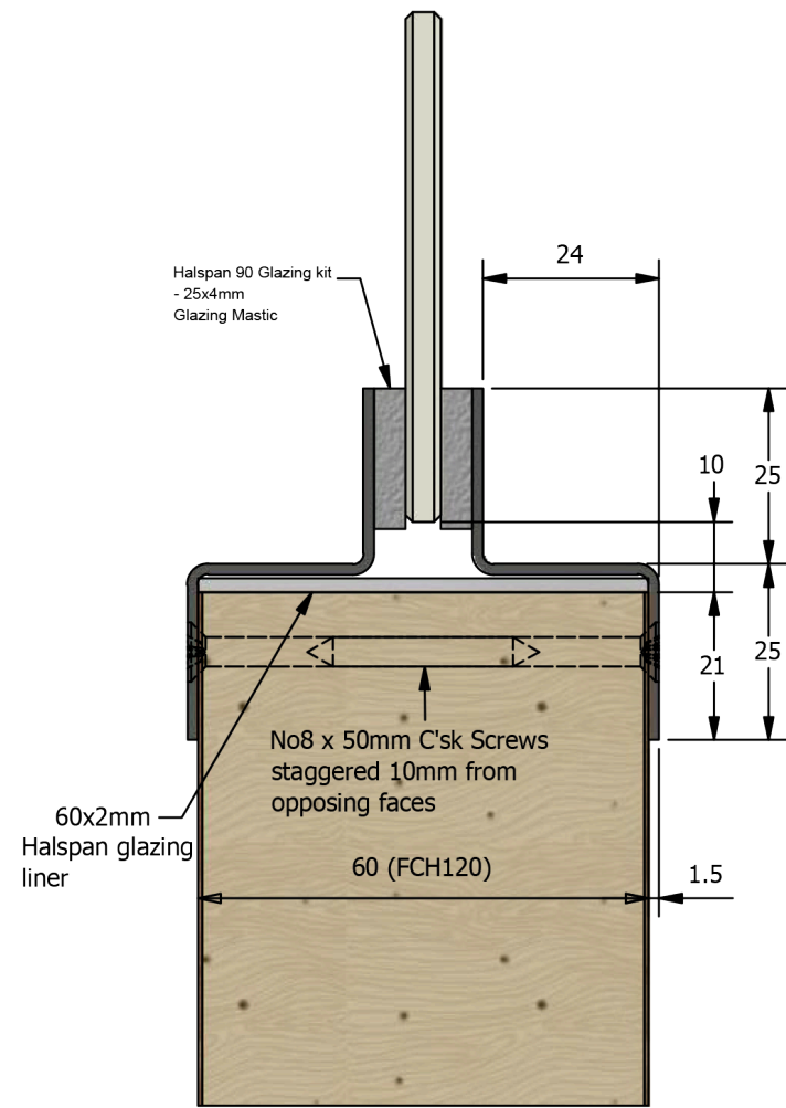
5mm Fire Glass FD120 (FCH) (G120/1); S(120/1)
