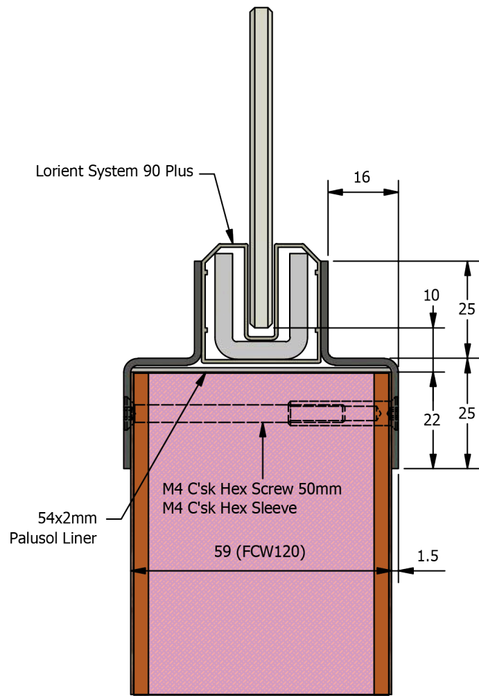
5mm Fire Glass FD120 (FCW) (G120/1); S(120/2)
