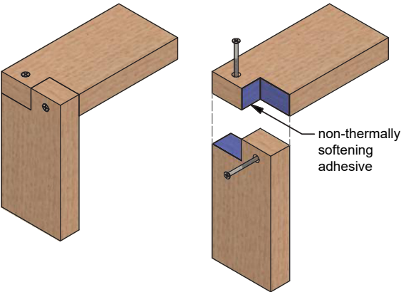
1 - Half-Lap Joint
