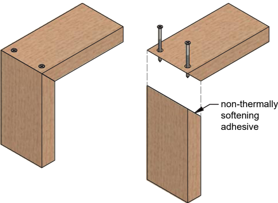
5 - Mitred Joint
