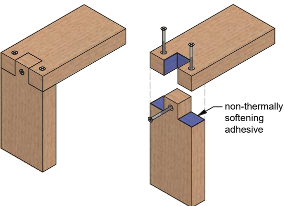
3 - Mortise & Tenon Open Joint
