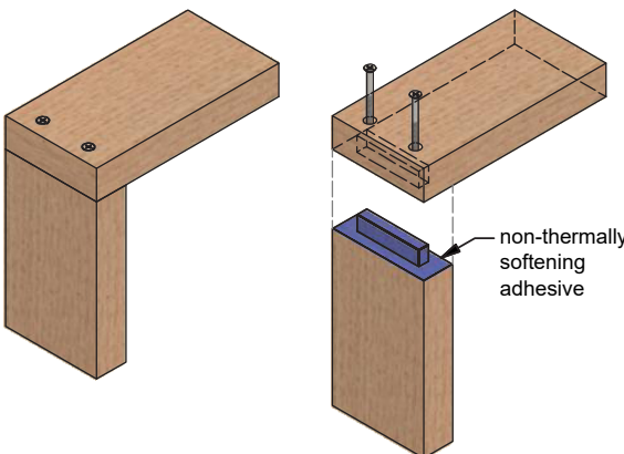
4 - Mortise & Tenon Stub Joint
