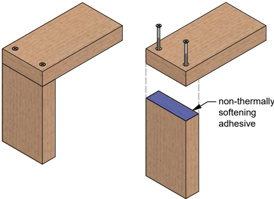
2 - Butt Joint
