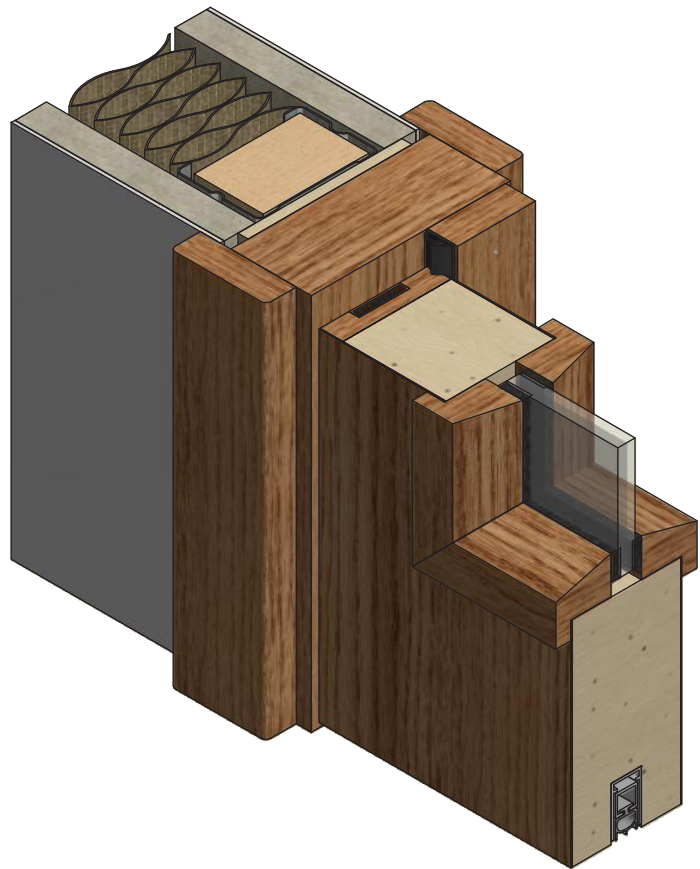
Isometric
