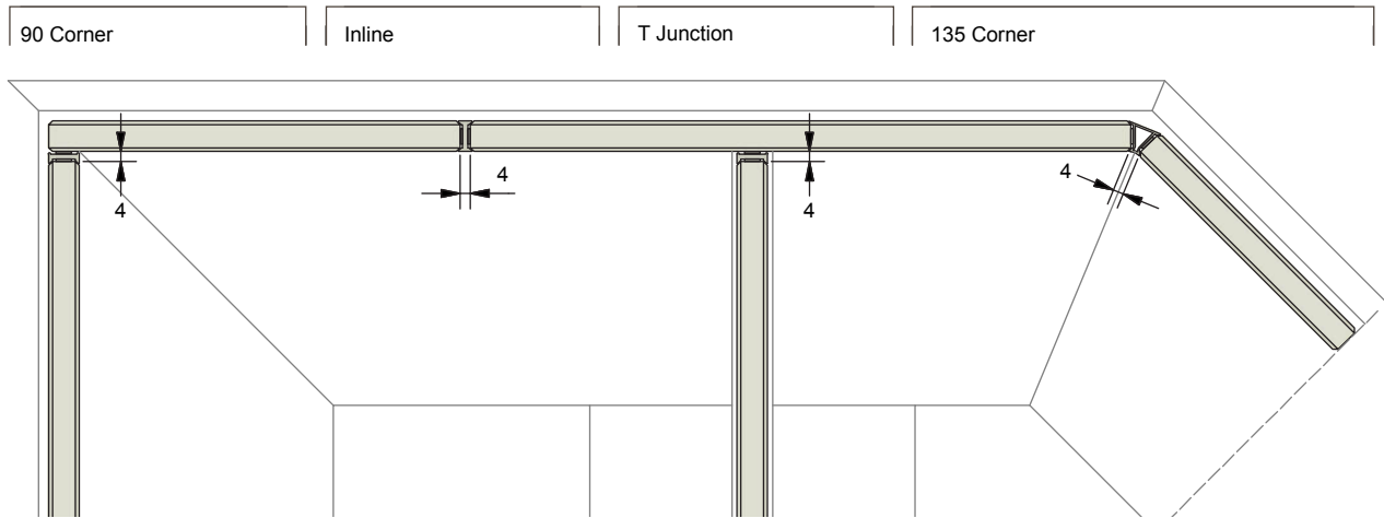
Glazed Joints (1:3)
