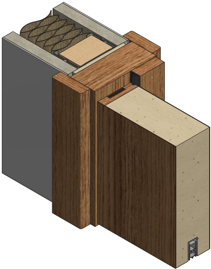
Isometric
