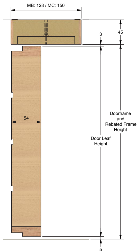
Head and Base (1:3)
