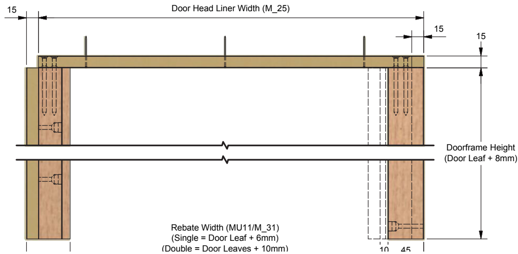
Doorframe Front View
