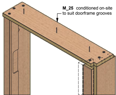
Doorframe Top Right Isometric
